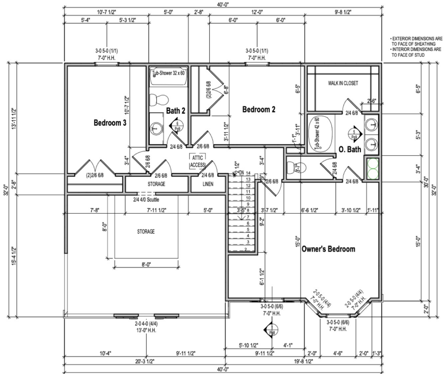
① 2nd Floor Plan - Elev B 1/8" = 1'-0"
