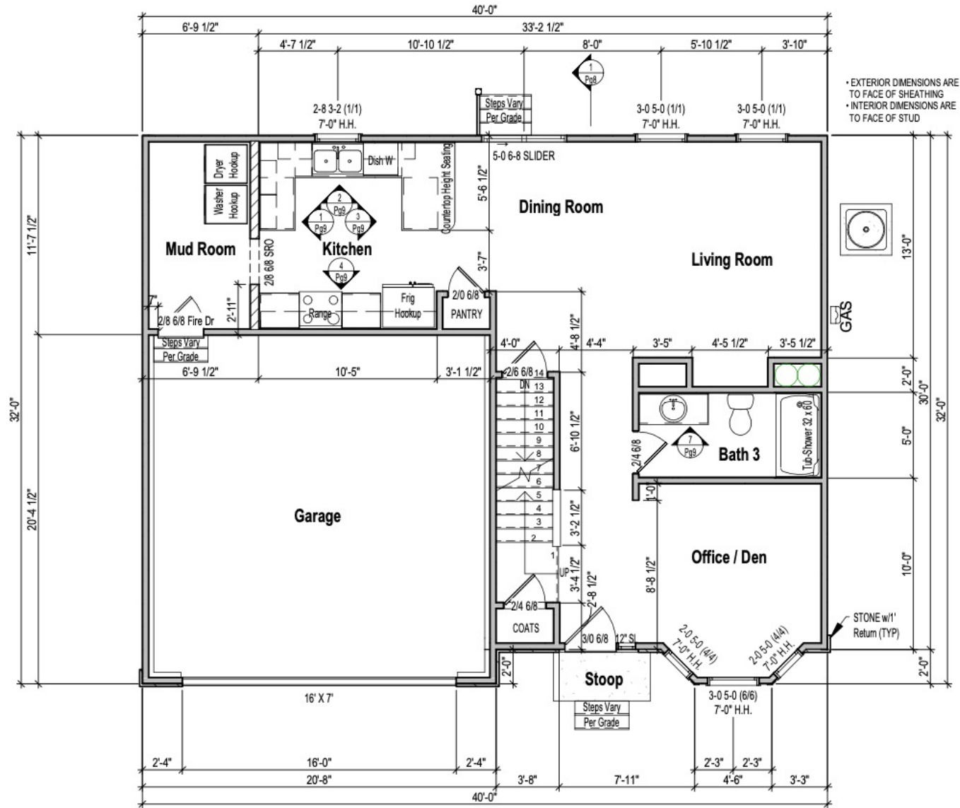
1 1st Floor Plan - Elev B 1/8" = 1'-0"
